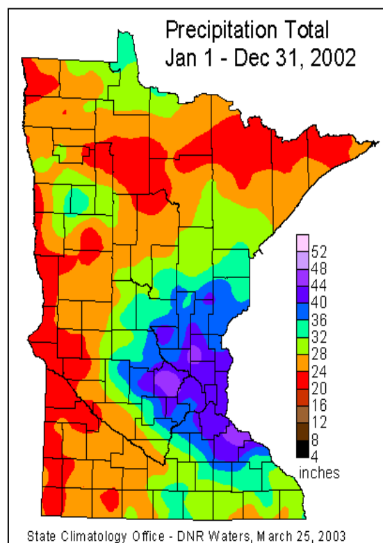
Figure 5. 2002 Precipitation totals
