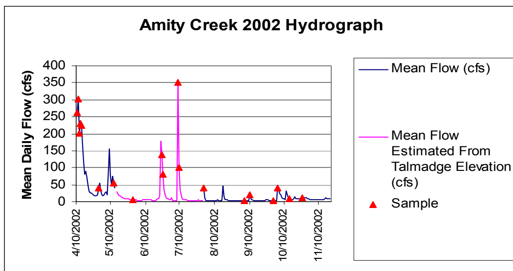
Figure 16. Amity Creek 2002 Hydrograph and Sampling dates
