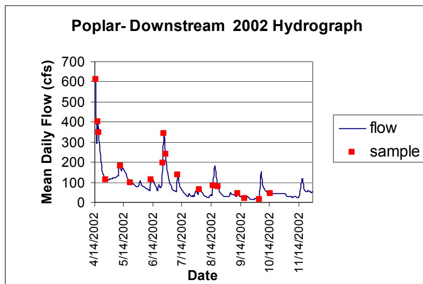
Figure 24. 2002 Poplar River ‘Downstream’ Hydrograph and Sampling Schedule
