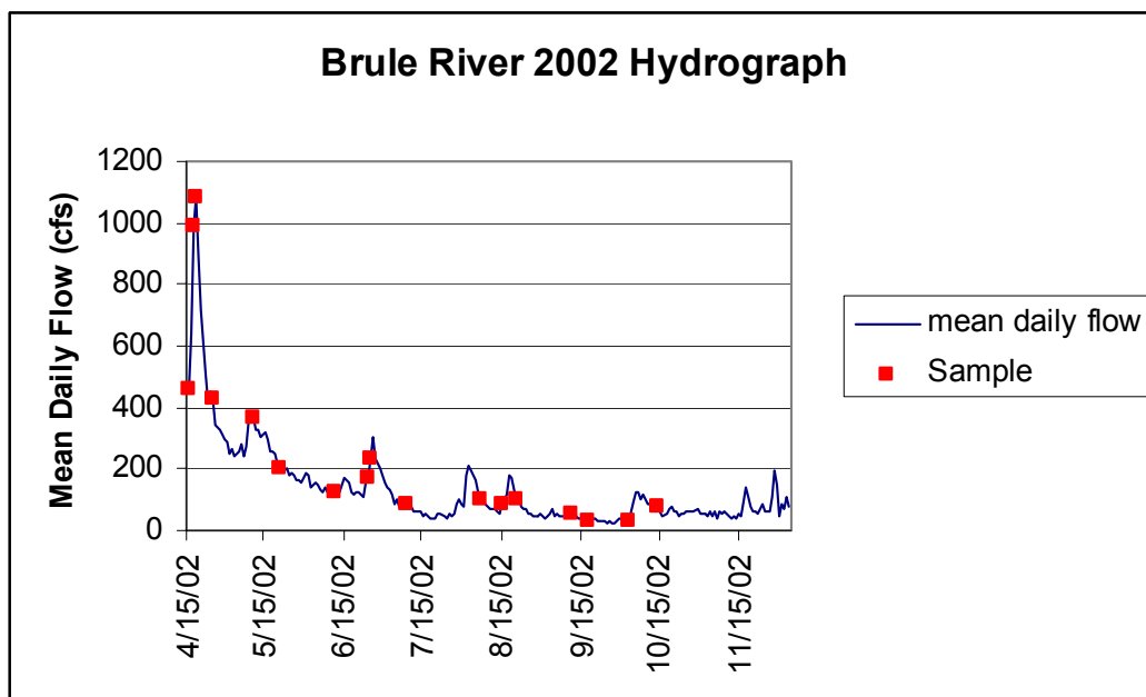
Figure 28. 2002 Brule River Hydrograph and Sampling Schedule
