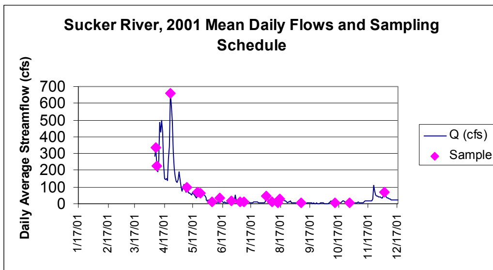
Figure 22. 2001 Sucker River Hydrograph and Sampling Schedule
