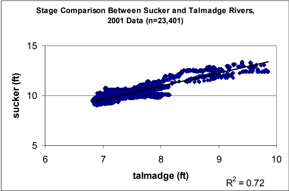
Figure 15. Stream stage comparisons between Sucker and Talmadge Rivers
